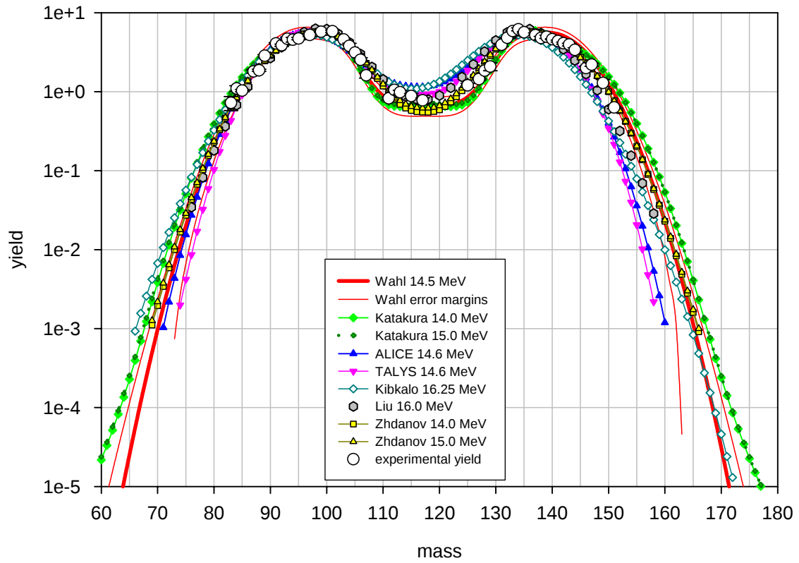
Benchmark A: ^{238}\text{U} around 14.5 MeV, post neutron emission yields
